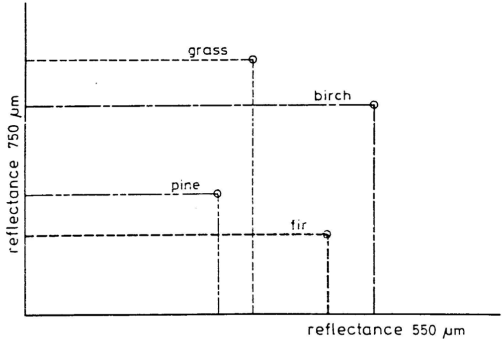
Figure 5 Relative reflected light of Pine, Fir, Birch and Grass across 1 and 3 SPOT band (wavelength 550 \mu\text{m} green and 750 \mu\text{m} near infrared)
